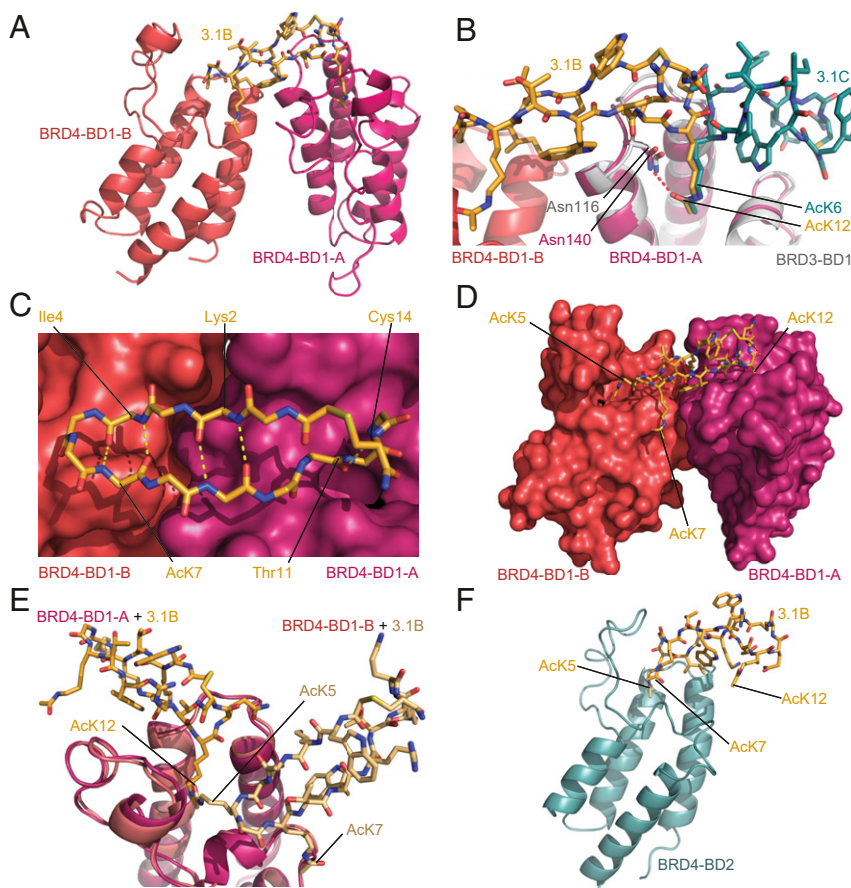
Fig. 3. 3.1B binds selectively to two BD1 domains through AcK-mediated interactions. (A) Ribbon diagram of the BRD4-BD1– 3.1B X-ray crystal structure (1.9-Å resolution, PDB ID code 6U74). The peptide is shown in orange and the two BDs bound to the peptide are shown in pink (BRD4-BD1-A) and coral red (BRD4-BD1-B). (B) Comparison of the binding modes of 3.1B (orange) and 3.1C (teal; bound to BRD3-BD1, gray). The two peptides insert an AcK into the AcK-binding pocket in identical conformations but otherwise use completely distinct binding modes. (C) Internal hydrogen bonding of 3.1B . Hydrogen bonds are indicated as yellow dashed lines. (D) Positions of the three AcK residues in the 3.1B complex. AcK5 is partially buried in the AcK binding site of the additional BD (BRD4-BD1-B; coral red), whereas AcK7 lies on the surface of that domain. (E) Comparison of the angle at which AcK12 and AcK5 enter the binding pocket in the two BD subunits in the 2:1 complex. A copy of the BRD4-BD1-B (coral red) has been overlaid with BRD4-BD1-A (pink) and a copy of 3.1B (pale orange) moved along with it. (F) Ribbon/stick representation of the X-ray crystal structure of the BRD4-BD2– 3.1B complex (2.6-Å resolution, PDB ID code 6U6L). The peptide is shown in orange and the BD is shown in blue.
